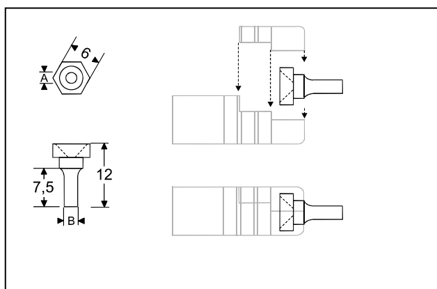
Manchon
